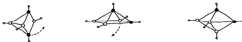
Fig. 18. The mode of interconversion between isomeric square pyramidal forms of \text{C}_2\text{B}_3\text{H}_5^{2-} .
