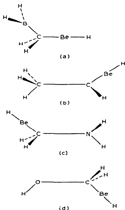
Fig. 10. The stable conformations of the molecules \text{HBeCH}_2\text{X} , where X = (a) \text{BH}_2 , (b) \text{CH}_3 , (c) \text{NH}_2 , (d) \text{OH} .
