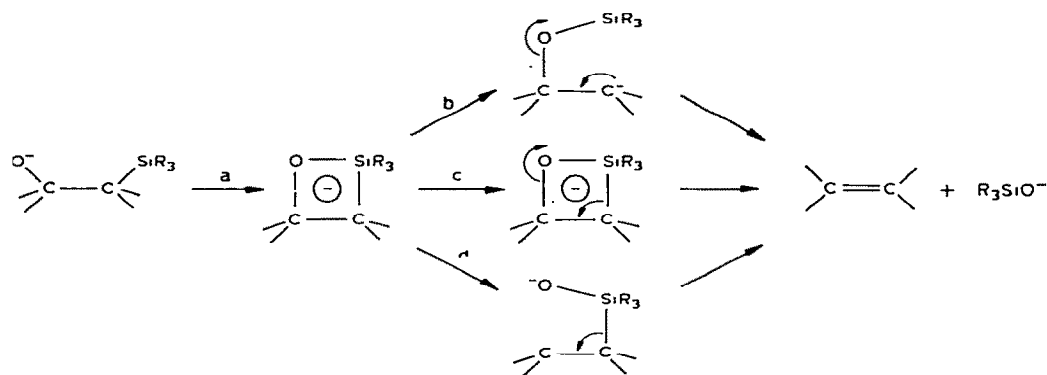
Fig. 41. Reaction paths in the decomposition of \text{SiH}_3\text{CH}_2\text{CH}_2\text{O}^- to \text{SiH}_3\text{O}^- and \text{C}_2\text{H}_4 : (a) initial formation of dihydrooxasiletanide anion; (b) nonconcerted decomposition of dihydrooxasiletanide anion via Si–C cleavage; (c) concerted decomposition of dihydrooxasiletanide; and (d) nonconcerted decomposition of dihydrooxasiletanide via C–O cleavage.
