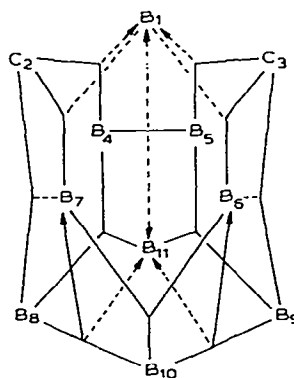
Fig. 28. The localised molecular orbitals for 1,6-C 2 B 8 H 10 .
