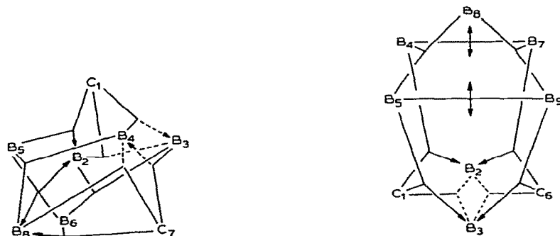
Fig. 25. The localised molecular orbitals for 1,7- C_2B_6H_8 .
