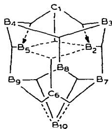
Fig. 28. The localised molecular orbitals for 1,6-C 2 B 8 H 10 .
