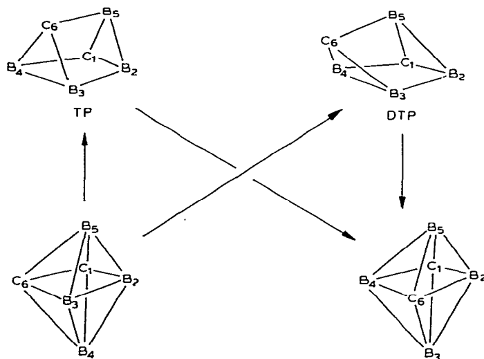
Fig. 21. The rearrangement schemes of 1,2- \text{C}_2\text{B}_4\text{H}_6 to 1,6- \text{C}_2\text{B}_4\text{H}_6 .
